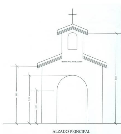
ALZADO PRINCIPAL
